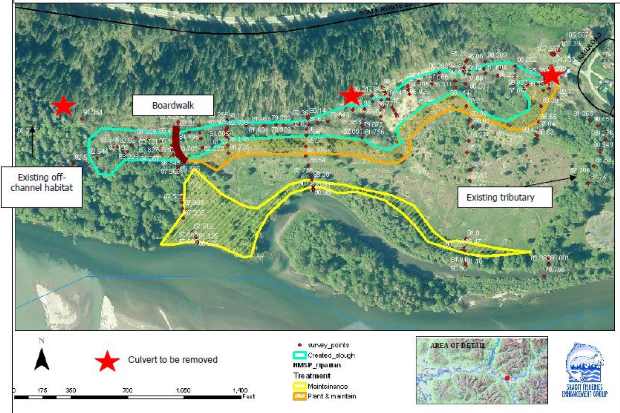
Figure 4. Proposed Howard Miller Steelhead Park off channel habitat enhancement project.
